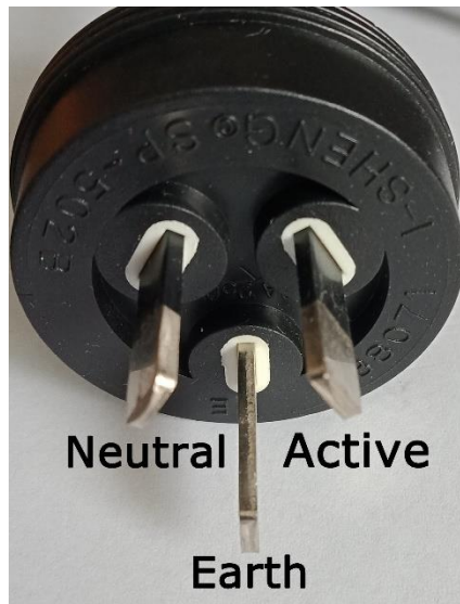
Figure 1: Three pin power plugs.
